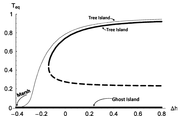
Figure 5. Stable ( solid ) and unstable ( dashed ) equilibrium states of tree biomass as a function of the elevation, \Delta h . In this analysis \Delta h is an assigned parameter, rather than being modeled as a function of T (equation (8)). The thick and the thin lines correspond to the case with \beta' = 0.2 kg P ha ^{-1} and \beta' = 2.0 kg P ha ^{-1} , respectively. The other parameters are \alpha' = 9.75 kg P ha ^{-1} (that is, \alpha = 0.68 kg P ha ^{-1} y ^{-1} , k = 0.07 y ^{-1} ) whereas a , b , c , and d_0 are as in Figure 3.
