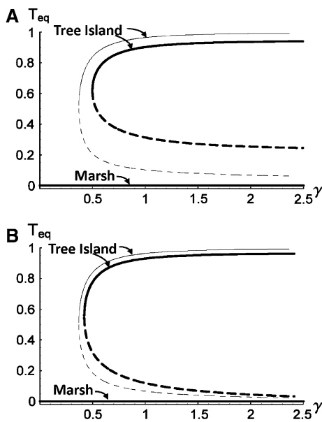
Figure 6. Stable (solid) and unstable (dashed) equilibrium states of tree biomass as a function of the parameter, \gamma expressing the relative importance of soil formation and soil erosion. In this analysis \Delta h is modeled as a function of T (equation (8)). Thus, at equilibrium low values of T correspond to low elevation (that is, more flooded) sites. A \beta' = 0.2 kg P ha -1 and B \beta' = 2.0 kg P ha -1 . The other parameters are \alpha' = 9.75 kg P ha -1 (thick lines) and \alpha' = 30 kg P ha -1 (thin lines) whereas a , b , c , and d_0 are as in Figure 3.
