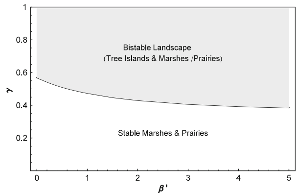
Figure 7. Domains of the parameter space corresponding to stable marsh and bistable island/marsh conditions.
