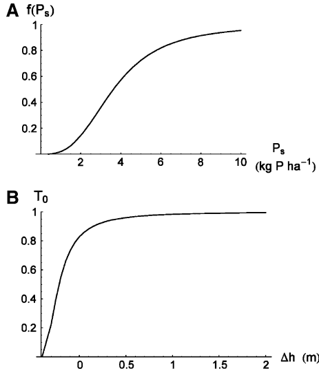
Figure 3. A A plot of equation (3) calculated with a = 0.21 and b = 3 ; B a plot of equation (4) calculated with c = 30 \text{ m}^{-1} and d_0 = -0.40 \text{ m} .
