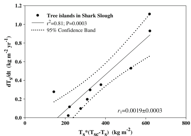
Figure 4. The rate of tree growth ( dT_s/dt ) measured with dendrometers on 10 islands in Shark Slough (Everglades National Park) is dependent on the existing standing tree biomass ( T_s ) and the difference between T_s and the carrying capacity of islands ( T_{cs} ). For this analysis, T_{cs} is estimated at 50 \text{ kg ha}^{-1} , approximately 1.5 times the maximum biomass found on these islands. The slope of the expression is equivalent to r_1 in equation (1). See Table 1 for island locations and dendrometer species lists. Regression statistical tests: Durbin–Watson Statistic = 2.058 (passed), Shapiro–Wilk normality test P = 0.123 (passed); W -statistic = 0.88 ( P = 0.05 ); Constant variance test P = 0.123 (passed).
