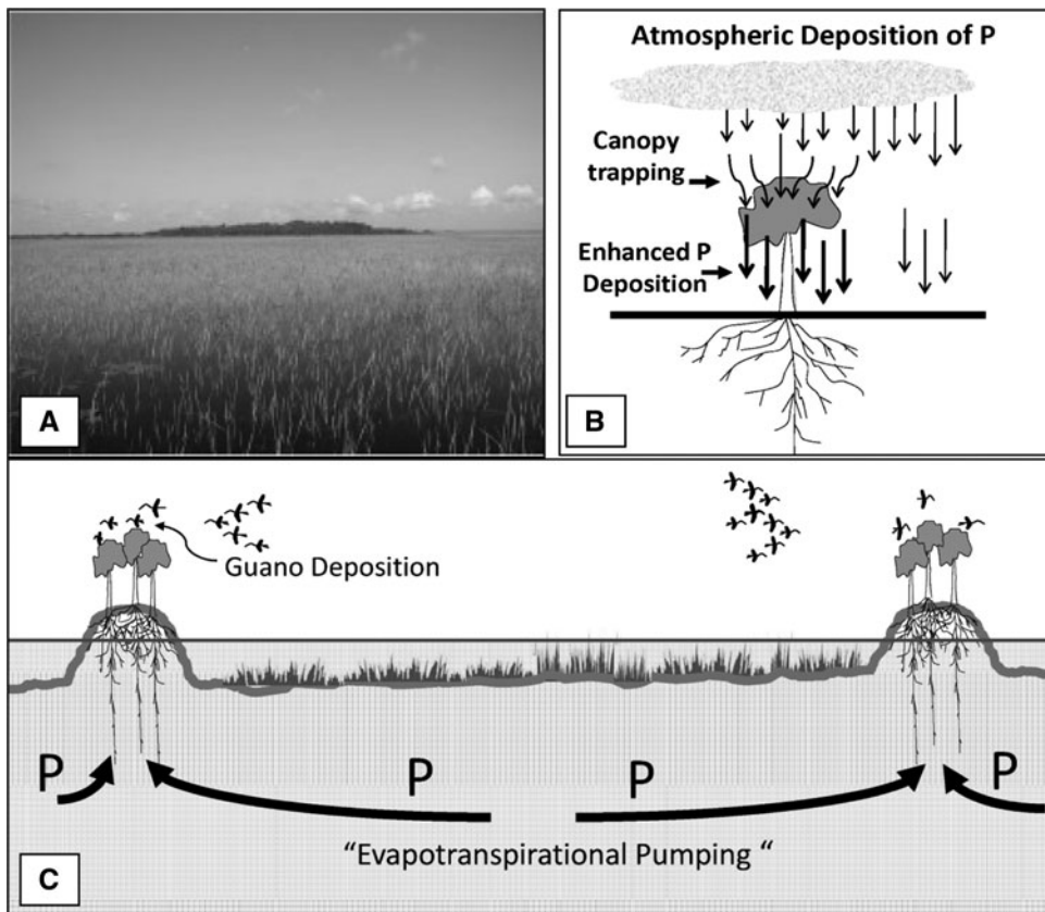
Figure 1. A A profile view of a tree island surrounded by grasses and herbaceous marsh species in Everglades, National Park. Schematic representation of the P enrichment due to the deposition feedback (B), and guano deposition or evapotranspirational pumping (C).
