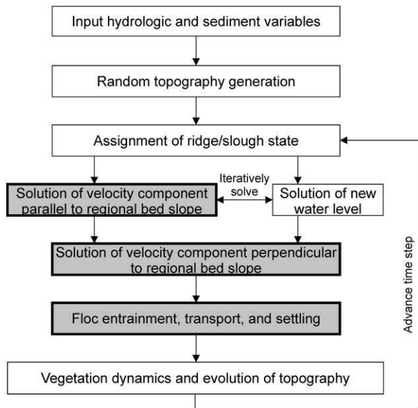
Fig. 2. Modularized structure of the RASCAL model. Different modules, which collectively simulate interactions among flow, sediment transport, and vegetation dynamics, operate over different timescales. Boxes depicted in gray operate only during pulses of high flow in which bed shear stresses are sufficient to entrain sediment. Other boxes operate continuously. A complete model time step is defined as the period of time over which the topography remains approximately static with respect to evolution of the flow field.
