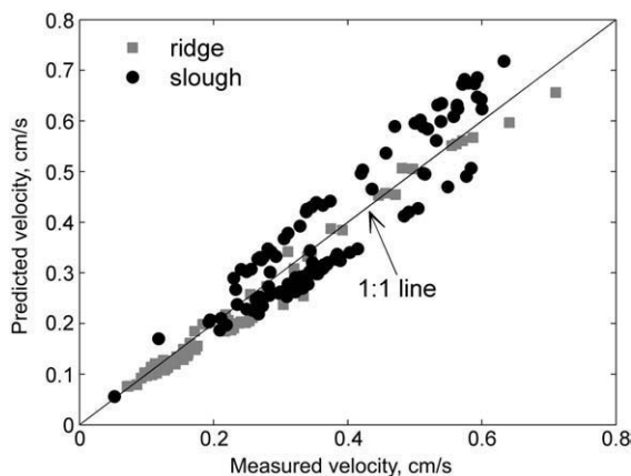
Fig. 4. Measured versus predicted mean longitudinal velocities in a relatively well-preserved part of the ridge and slough landscape. Daily average velocities were measured over two wet seasons with an acoustic Doppler velocimeter, as described in Harvey et al. (2009). Simultaneous measurements of water-surface slope and flow depths and one-time measurement of vegetation community architectures provided the inputs needed for this RASCAL model run.
