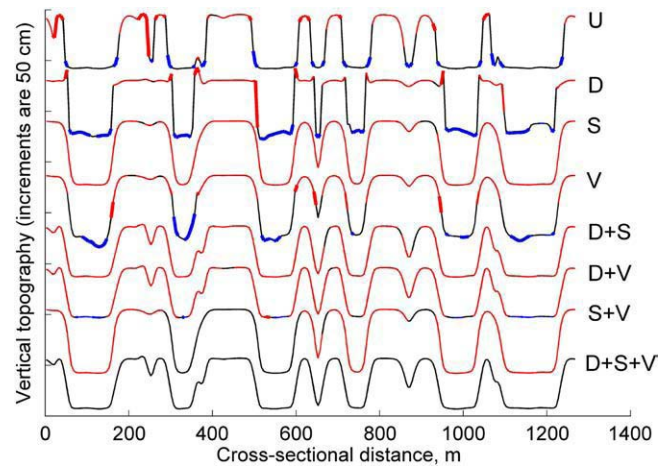
Fig. 8. Cross-sectional profiles across the unperturbed (U) landscape at 41% high-resistance vegetation coverage and perturbed landscapes at 60% high-resistance vegetation coverage. (D = decreased water depth, S = decreased water-surface slope, V = increased vegetative drag in low-resistance patches due to invasion by high-resistance vegetation.) Cross-sections are plotted with respect to an arbitrary datum for ease of viewing. Red and blue segments show zones of sediment deposition and erosion, respectively, where the thickness of the line is related to the magnitude of the bed sediment flux. Thin red and blue lines indicate immeasurably low rates of bed sediment flux.
